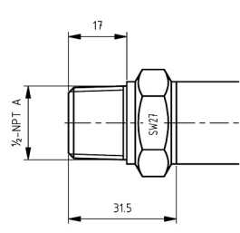
Fig. 8 - 1/2 NPT A
